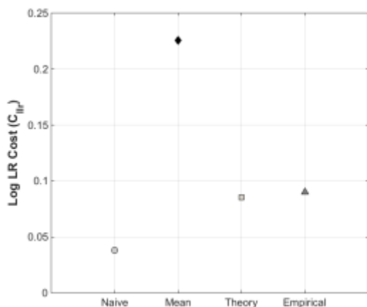
Figure 2: C_{llr} for the four systems using front-end techniques to account for correlations.
